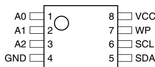
8-lead TSSOP
