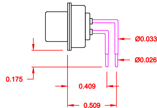
SIGNAL CONTACTS
