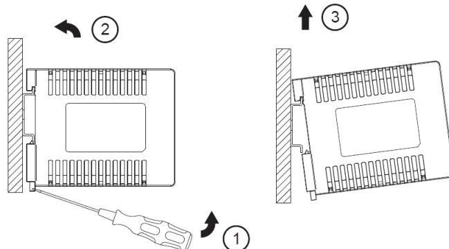
Fig. 2.2 Dismounting
