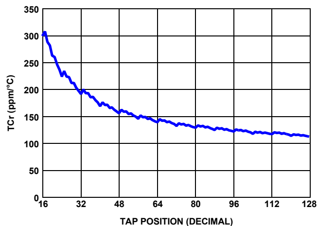
FIGURE 9. 10k TCr vs TAP POSITION
