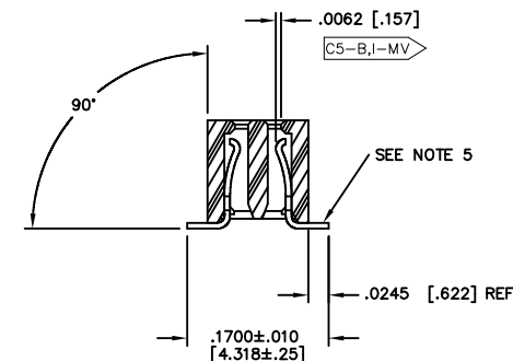
SECT "B-B"
