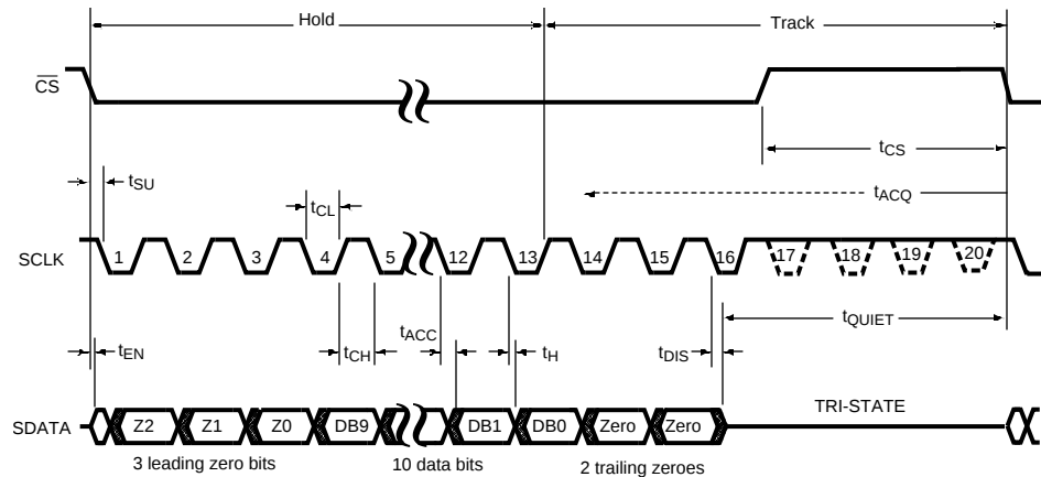
Figure 3. ADC101S101 Serial Timing Diagram
