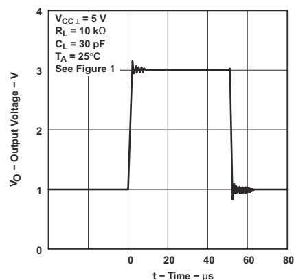
Figure 6-38. TLE2024 Voltage-Follower Large-Scale Pulse Response
