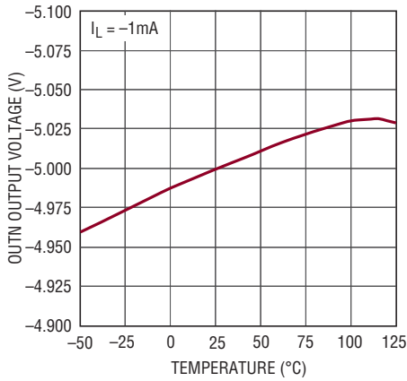
LT3032-5 OUTN Output Voltage
