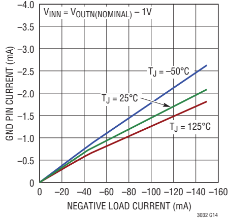
Negative Side GND Pin Current vs I_{LOAD}
