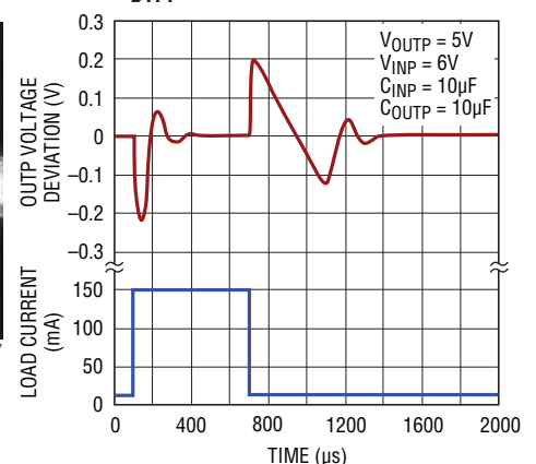
OUTP Transient Response, C_BYP = 0
