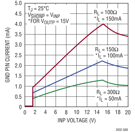
LT3032 Negative Side GND Pin Current
