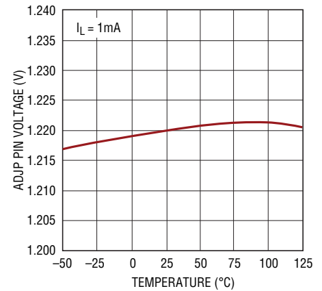
LT3032 ADJP Pin Voltage
