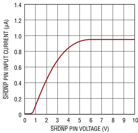
\overline{SHDNP} Pin Input Current
