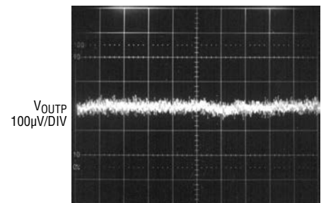
OUTP 10Hz to 100kHz Output Noise, C_BYP = 0.01µF
