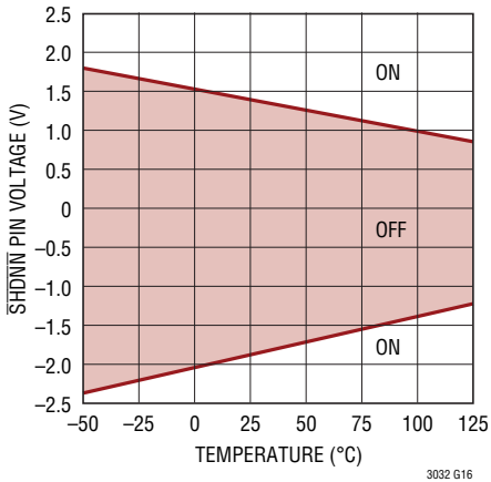
\overline{SHDNN} Pin Thresholds
