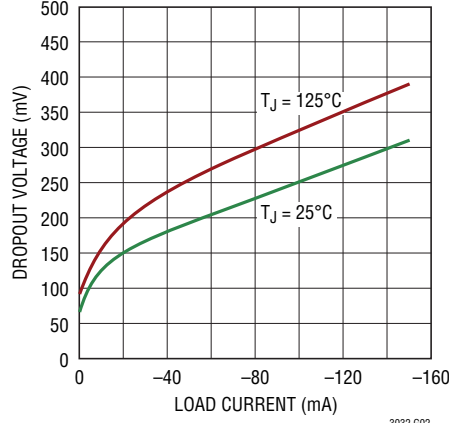
INN-to-OUTN Typical Dropout Voltage
