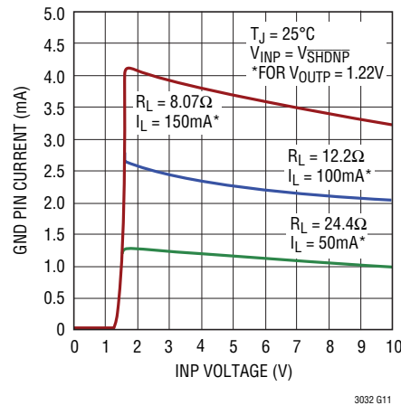
LT3032 Positive Side GND Pin Current
