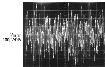
OUTP 10Hz to 100kHz Output Noise, C_BYP = 0
