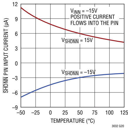
\overline{SHDNN} Pin Input Current
