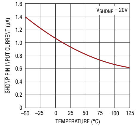
\overline{SHDNP} Pin Input Current
