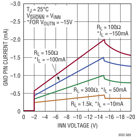
LT3032-15 Negative Side GND Pin Current
