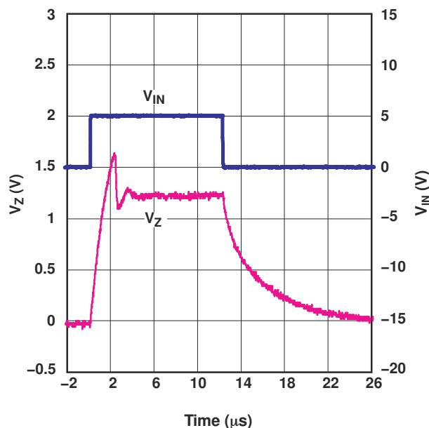
Figure 5-3. Start-Up Characteristics
