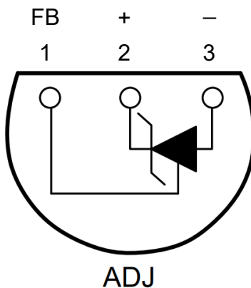
Figure 4-6. LP Package 3-Pin TO-92 Bottom View
