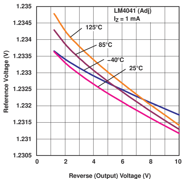
Figure 5-4. Reference Voltage vs Reverse (Output) Voltage (for Different Temperatures)
