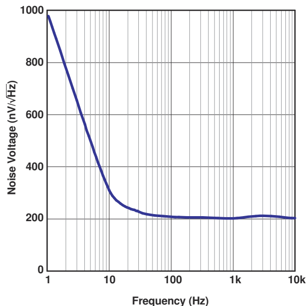
Figure 5-2. Noise Voltage vs Frequency
