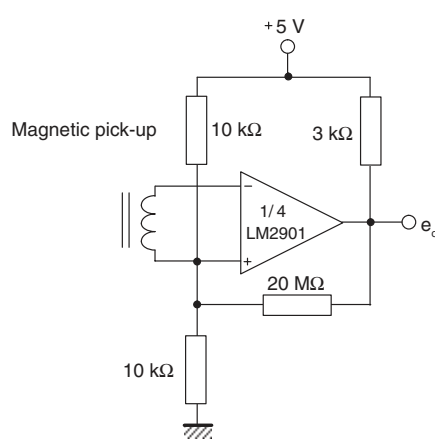
Figure 13. Transducer amplifier
