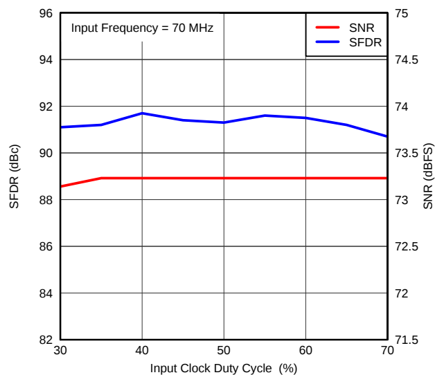
Figure 64. PERFORMANCE vs CLOCK DUTY CYCLE (70 MHz)
