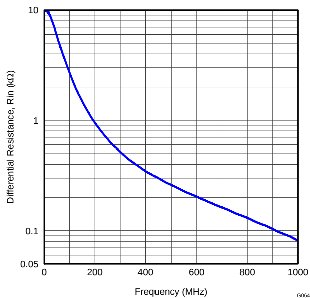
Figure 83. ADC Analog Input Resistance ( R_{IN} ) Across Frequency
