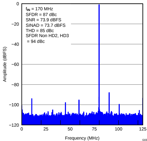
Figure 40. FFT FOR 170-MHz INPUT SIGNAL (2.5-V PP Full-Scale)
