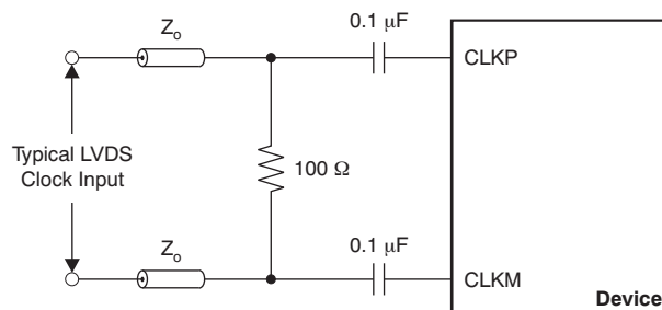
Figure 88. LVDS Clock Driving Circuit
