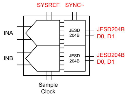
Figure 93. JESD204B Interface
