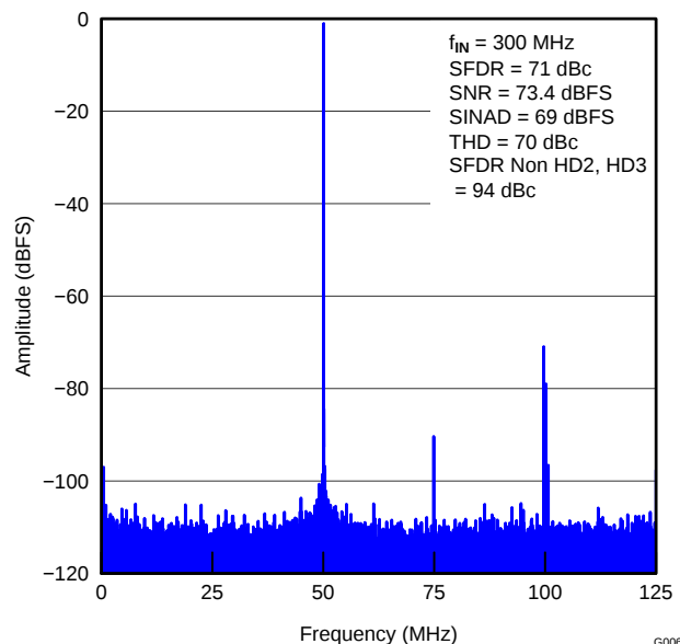
Figure 11. FFT FOR 300-MHz INPUT SIGNAL ( 2.5\text{-}V_{PP} Full-Scale)
