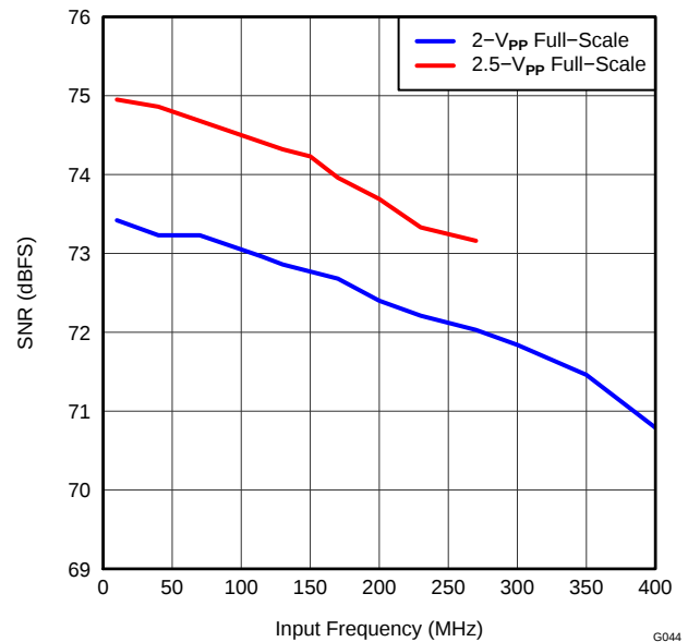
Figure 49. SIGNAL-TO-NOISE RATIO vs INPUT FREQUENCY
