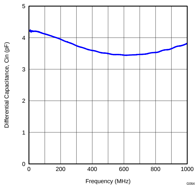
Figure 84. ADC Analog Input Capacitance ( C_{IN} ) Across Frequency
