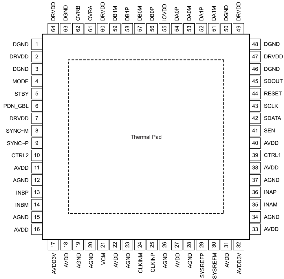
RGC PACKAGE QFN-64 (Top View)
