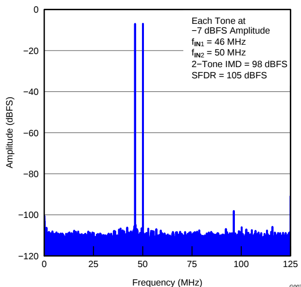
Figure 12. FFT FOR TWO-TONE INPUT SIGNAL ( -7\text{ dBFS} at 46 MHz and 50 MHz)
