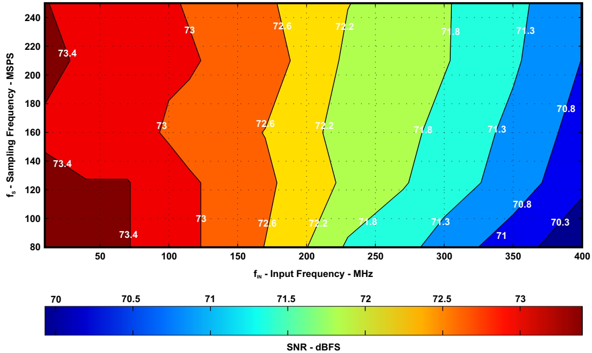
Figure 76. 0-dB GAIN (SNR, ADS42JB49)
