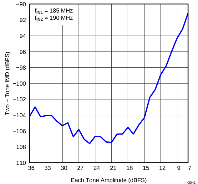
Figure 47. INTERMODULATION DISTORTION vs INPUT AMPLITUDE (185 MHz and 190 MHz)
