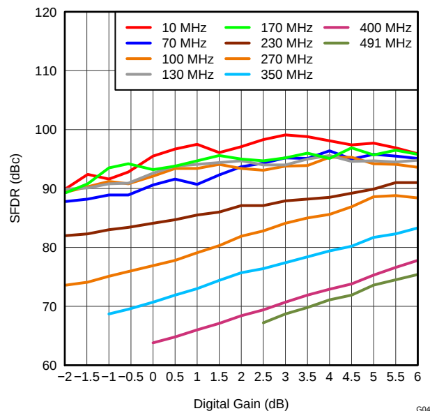
Figure 50. SPURIOUS-FREE DYNAMIC RANGE vs DIGITAL GAIN
