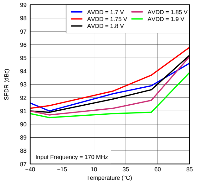
Figure 56. SPURIOUS-FREE DYNAMIC RANGE vs AVDD SUPPLY AND TEMPERATURE (170 MHz)
