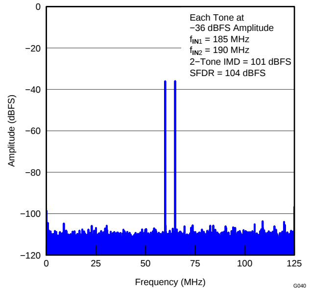
Figure 45. FFT FOR TWO-TONE INPUT SIGNAL (-36 dBFS at 185 MHz and 190 MHz)
