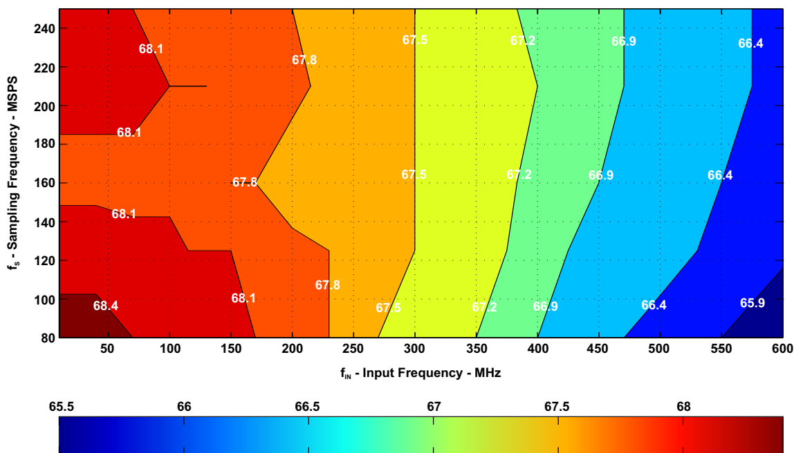
Figure 75. 6-dB GAIN (SNR, ADS42JB69)
