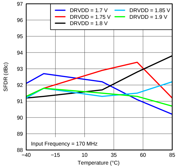
Figure 30. SPURIOUS-FREE DYNAMIC RANGE vs DRVDD SUPPLY AND TEMPERATURE (170 MHz)
