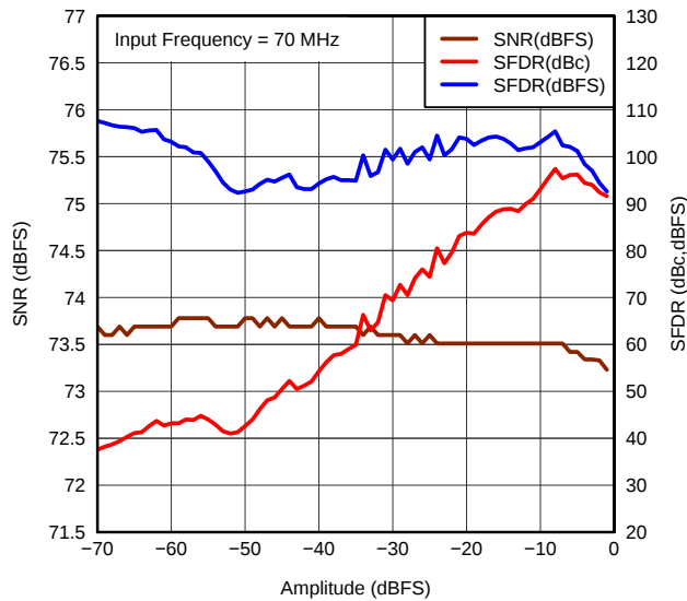
Figure 52. PERFORMANCE vs INPUT AMPLITUDE (70 MHz)
