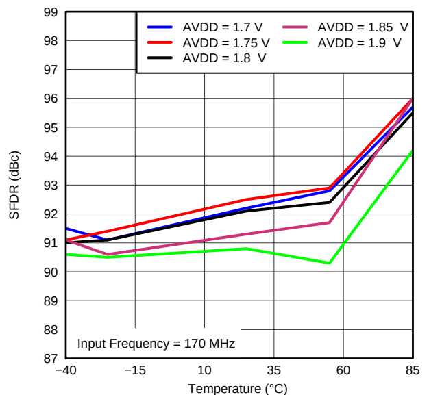
Figure 26. SPURIOUS-FREE DYNAMIC RANGE vs AVDD SUPPLY AND TEMPERATURE (170 MHz)
