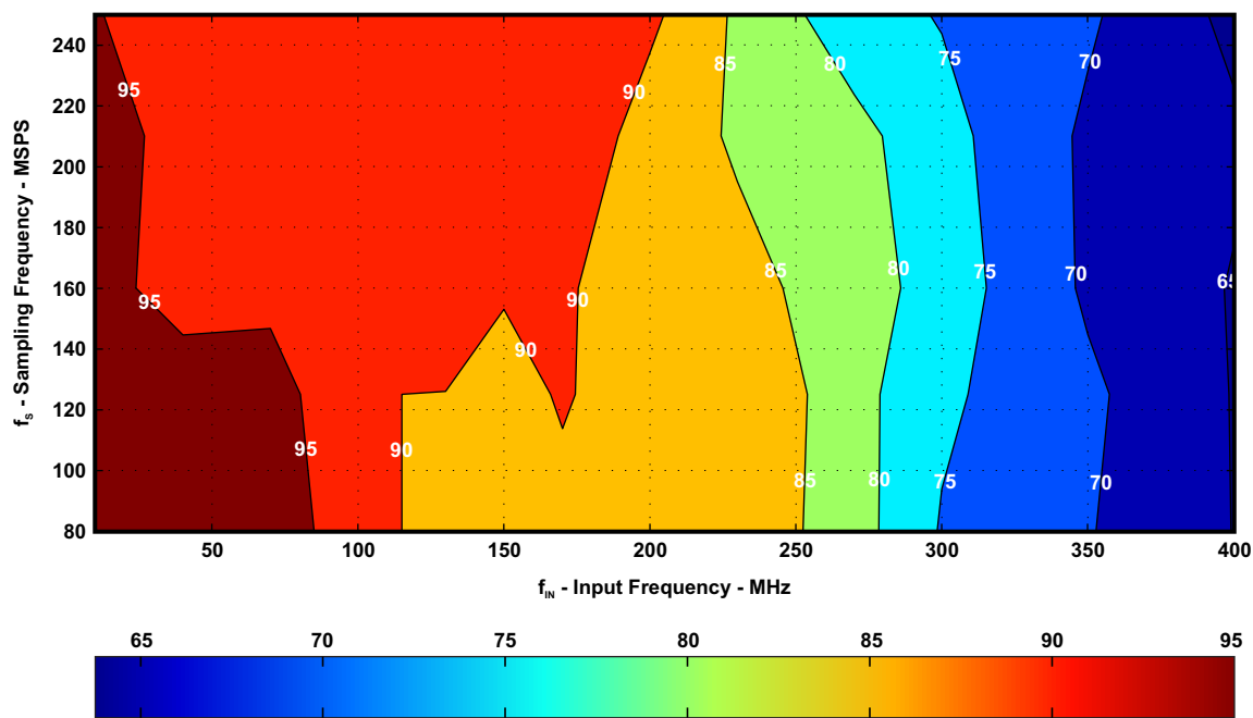
Figure 72. 0-dB GAIN (SFDR)
