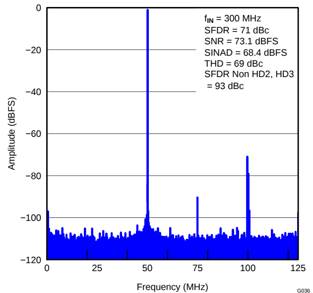
Figure 41. FFT FOR 300-MHz INPUT SIGNAL (2.5-V PP Full-Scale)
