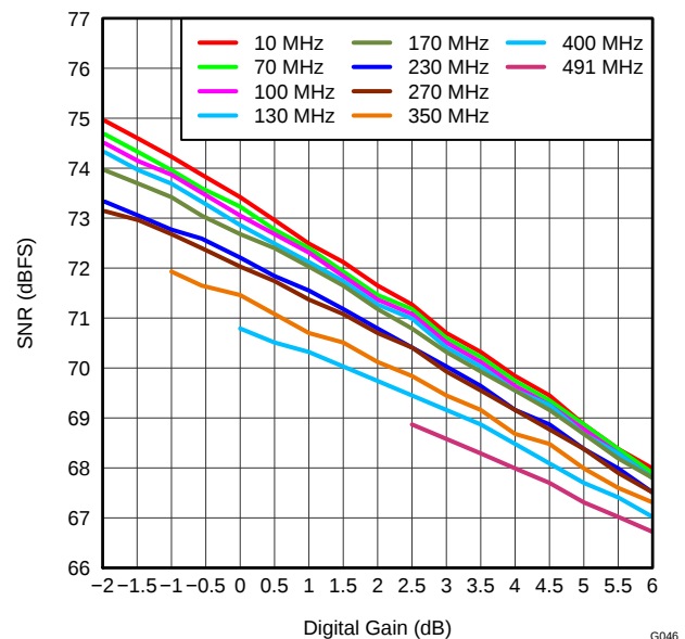
Figure 51. SIGNAL-TO-NOISE RATIO vs DIGITAL GAIN
