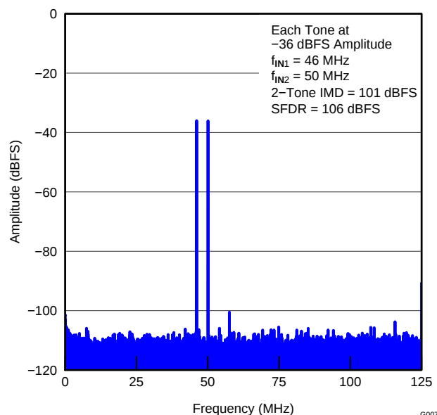
Figure 13. FFT FOR TWO-TONE INPUT SIGNAL ( -36\text{ dBFS} at 46 MHz and 50 MHz)
