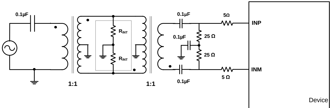
Figure 86. Drive Circuit for Input Frequencies > 250MHz
