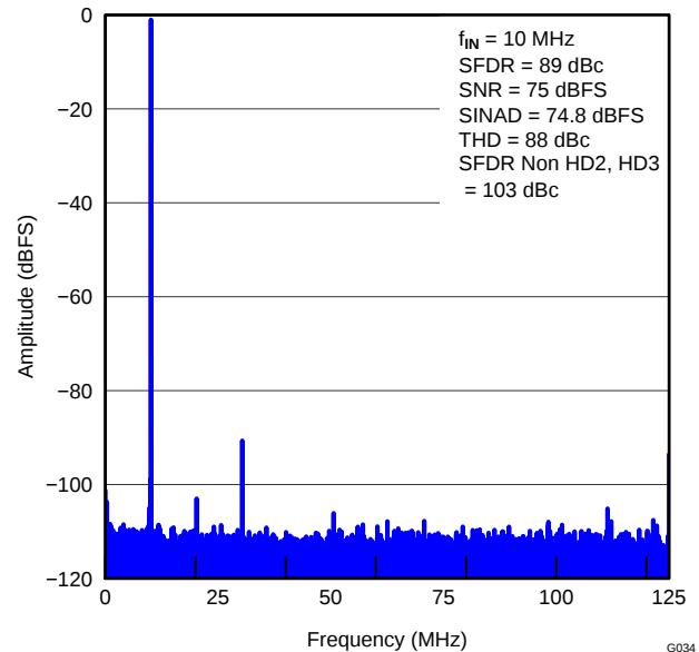
Figure 39. FFT FOR 10-MHz INPUT SIGNAL ( 2.5\text{-V}_{\text{PP}} Full-Scale)
