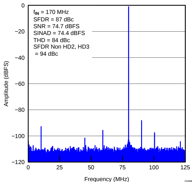
Figure 10. FFT FOR 170-MHz INPUT SIGNAL ( 2.5\text{-}V_{PP} Full-Scale)
