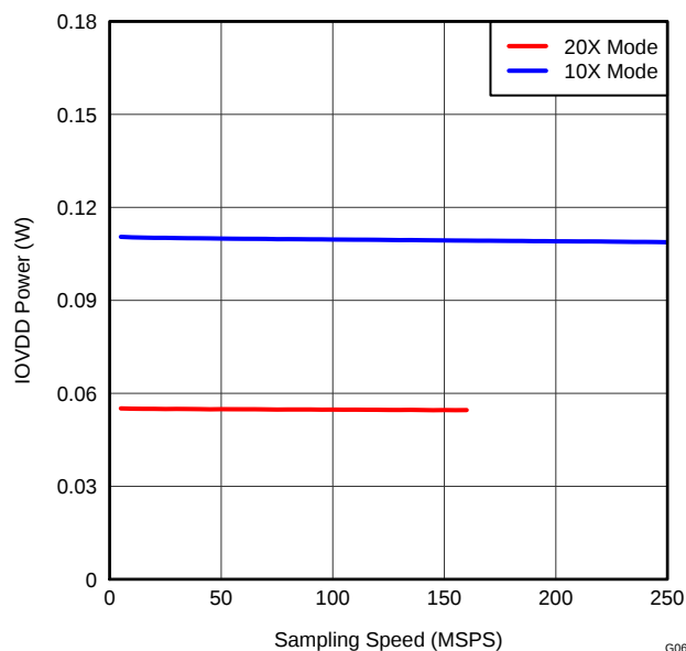
Figure 71. IOVDD POWER vs SAMPLING FREQUENCY G066
