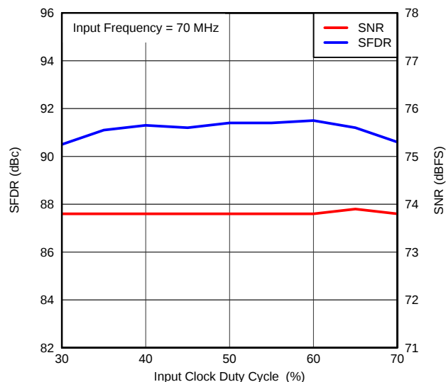
Figure 34. PERFORMANCE vs CLOCK DUTY CYCLE (70 MHz)
