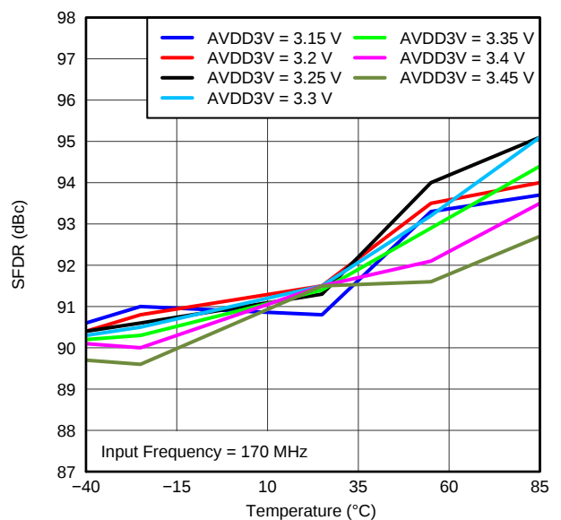
Figure 28. SPURIOUS-FREE DYNAMIC RANGE vs AVDD_BUF SUPPLY AND TEMPERATURE (170 MHz)
