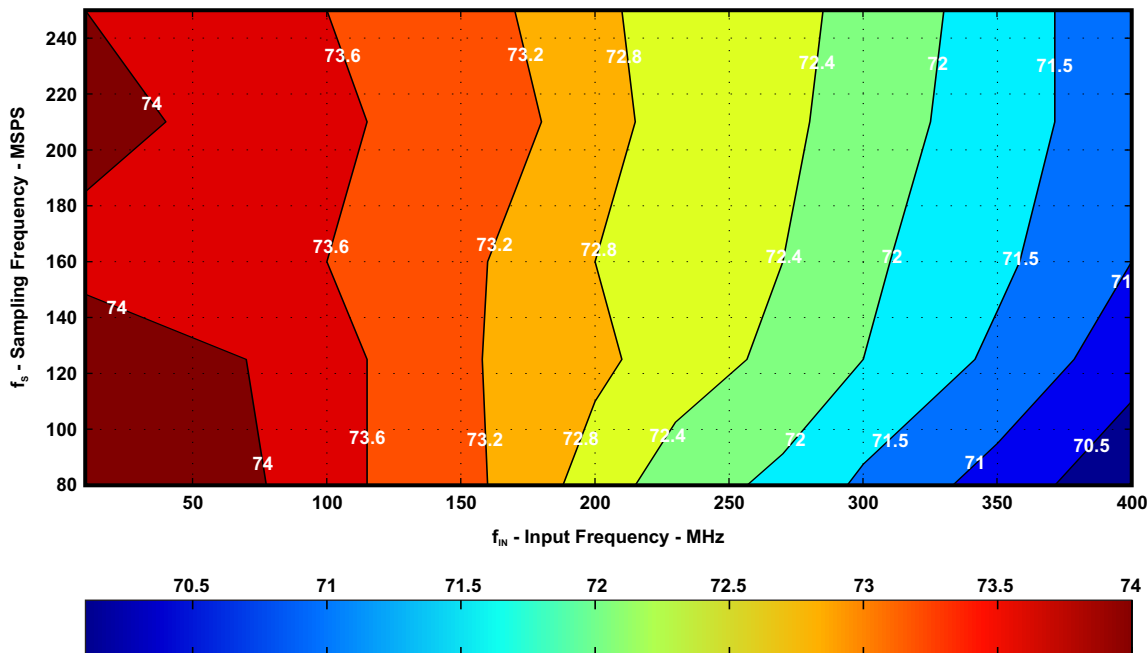
Figure 74. 0-dB GAIN (SNR, ADS42JB69)
