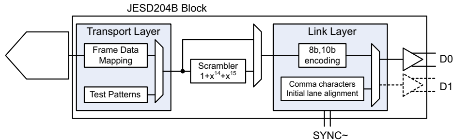
Figure 94. JESD204B Block
