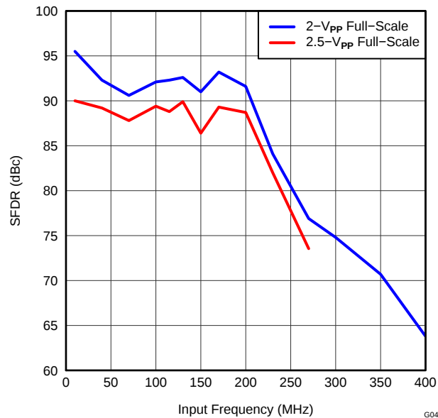
Figure 48. SPURIOUS-FREE DYNAMIC RANGE vs INPUT FREQUENCY
