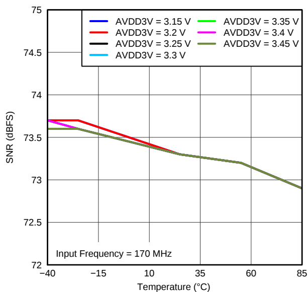
Figure 29. SIGNAL-TO-NOISE RATIO vs AVDD_BUF SUPPLY AND TEMPERATURE (170 MHz)
