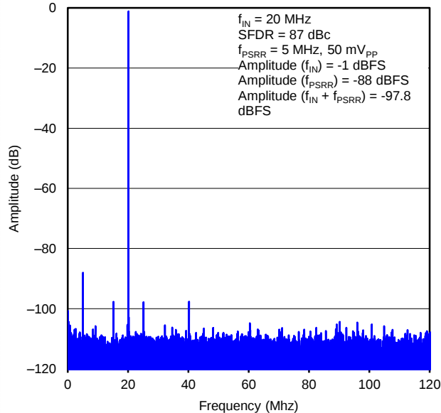
Figure 68. POWER-SUPPLY REJECTION RATIO FFT FOR AVDD SUPPLY
