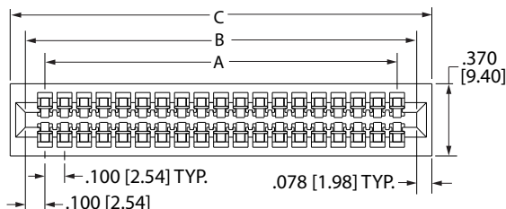
WITHOUT STANDOFFS
