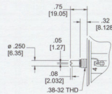
DETAIL OF SHAFT & BUSHING
