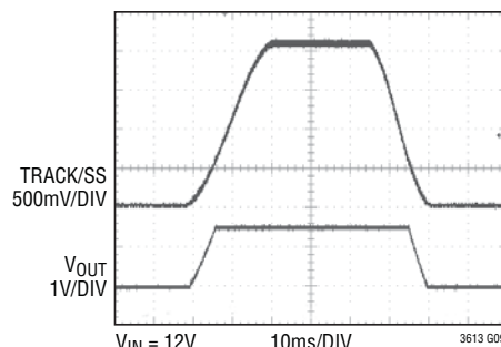
Output Tracking
