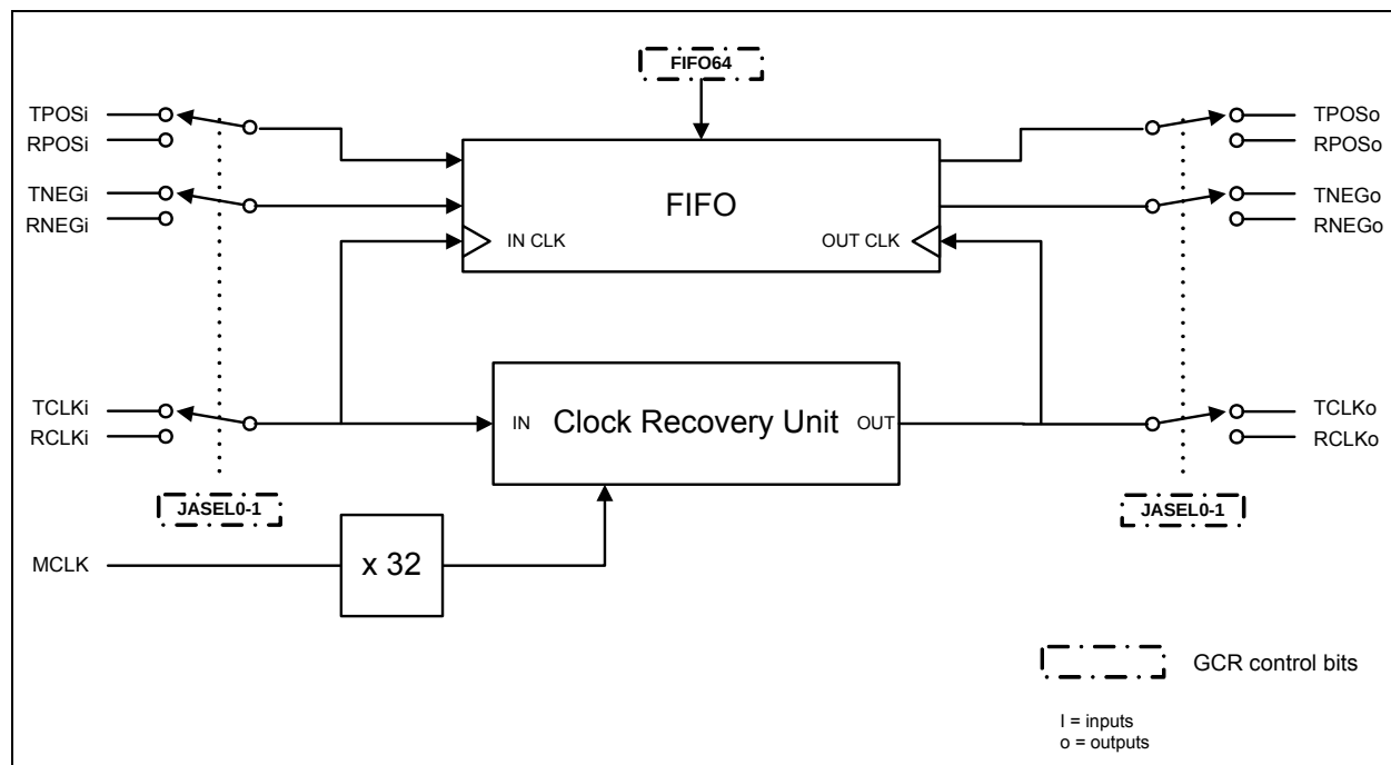
Figure 7 Jitter Attenuator
