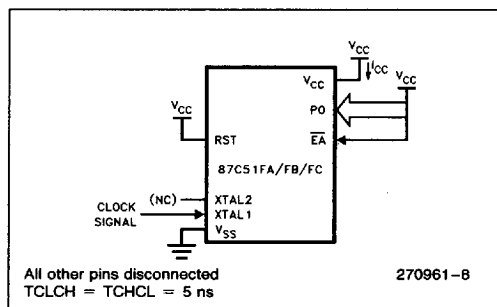
Figure 7. I_{CC} Test Condition, Active Mode
