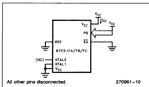
Figure 9. I_{CC} Test Condition, Power Down Mode. V_{CC} = 2.0\text{V to } 5.5\text{V} .
