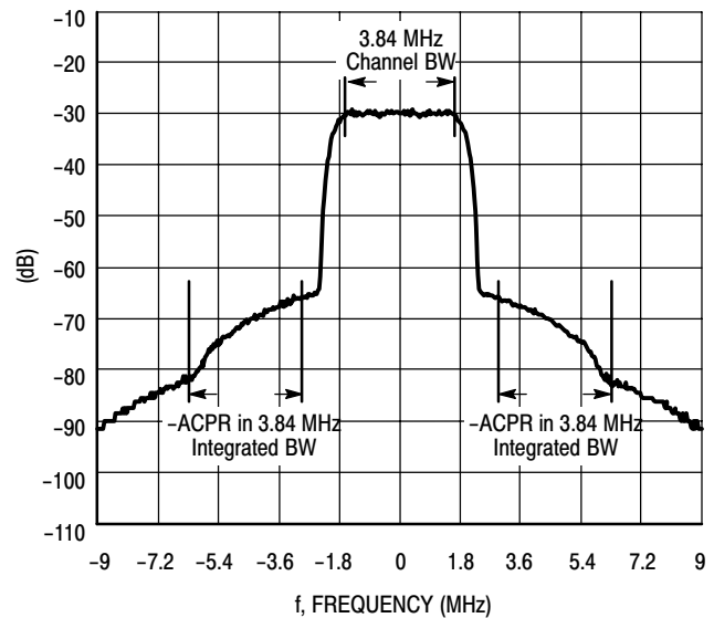
Figure 17. Single-Carrier W-CDMA Spectrum
