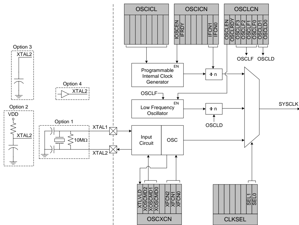
Figure 19.1. Oscillator Options
