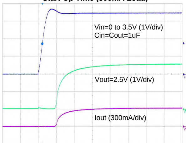
Start-Up Time (300mA Load)
