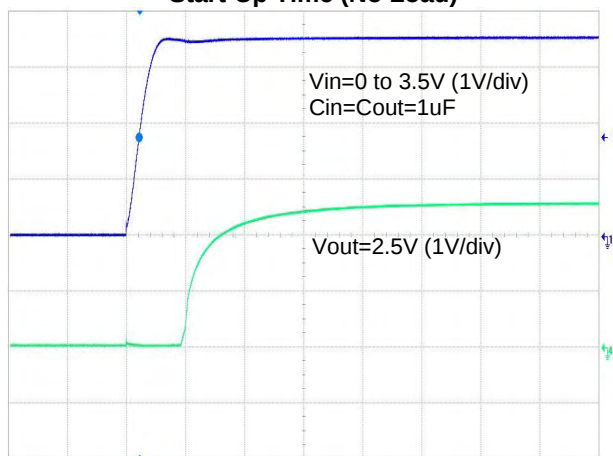
Start-Up Time (No Load)
