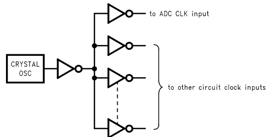
Figure 22. Isolating the ADC clock from Digital Circuitry.
