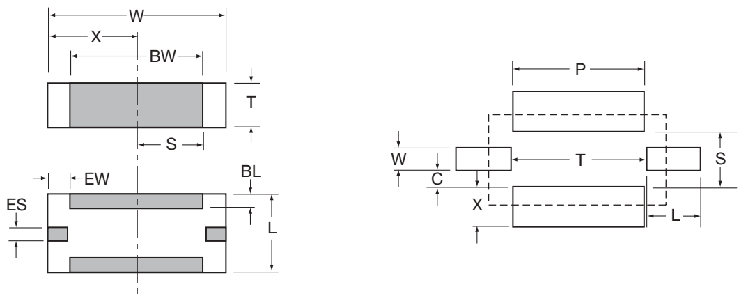
W3H1 - 0612 Style
