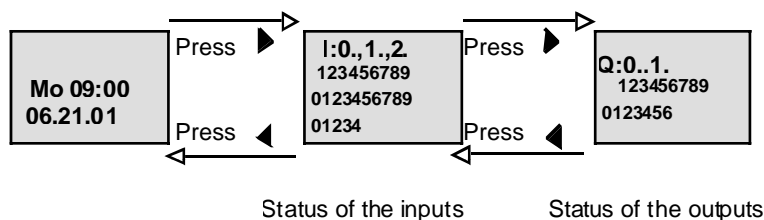
Display field of the IDEC SmartRelay in RUN mode
