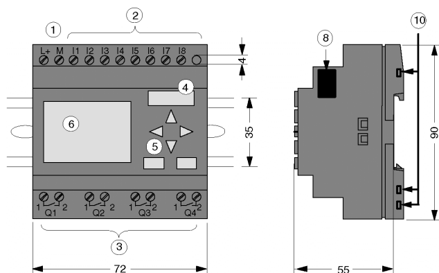
IDEC SmartRelay Basic (eg. FL1B-H12RCE)
