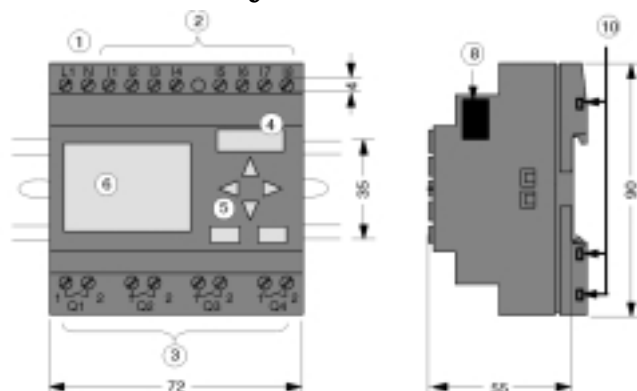
IDEC SmartRelay Basic (eg. FL1B-H12RCC)
