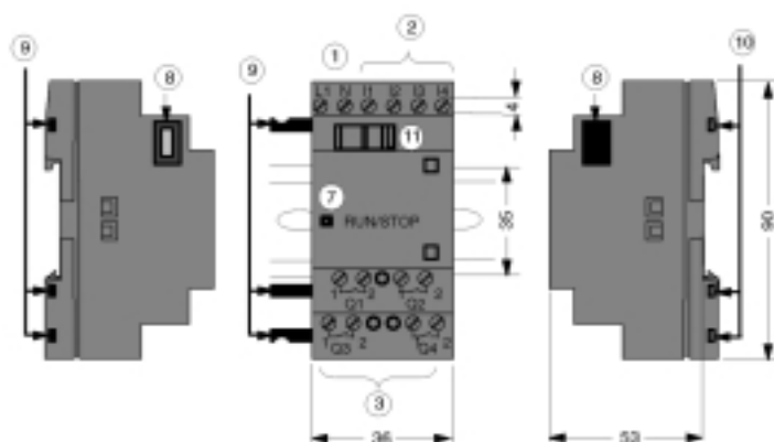
IDEC SmartRelay Expansion Module (eg. FL1B-M08C2R2)
