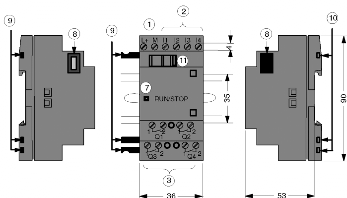
IDEC SmartRelay Expansion Module (eg. FL1B-M08B2R2)
