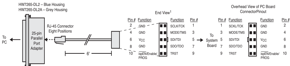
Figure 4. ispDOWNLOAD Cable In-System Programming Interface for the PC (HW7265-DL2 or HW7265-DL2A)
