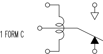
3.CONNECTION DIAGRAM(BOTTOM VIEW)
