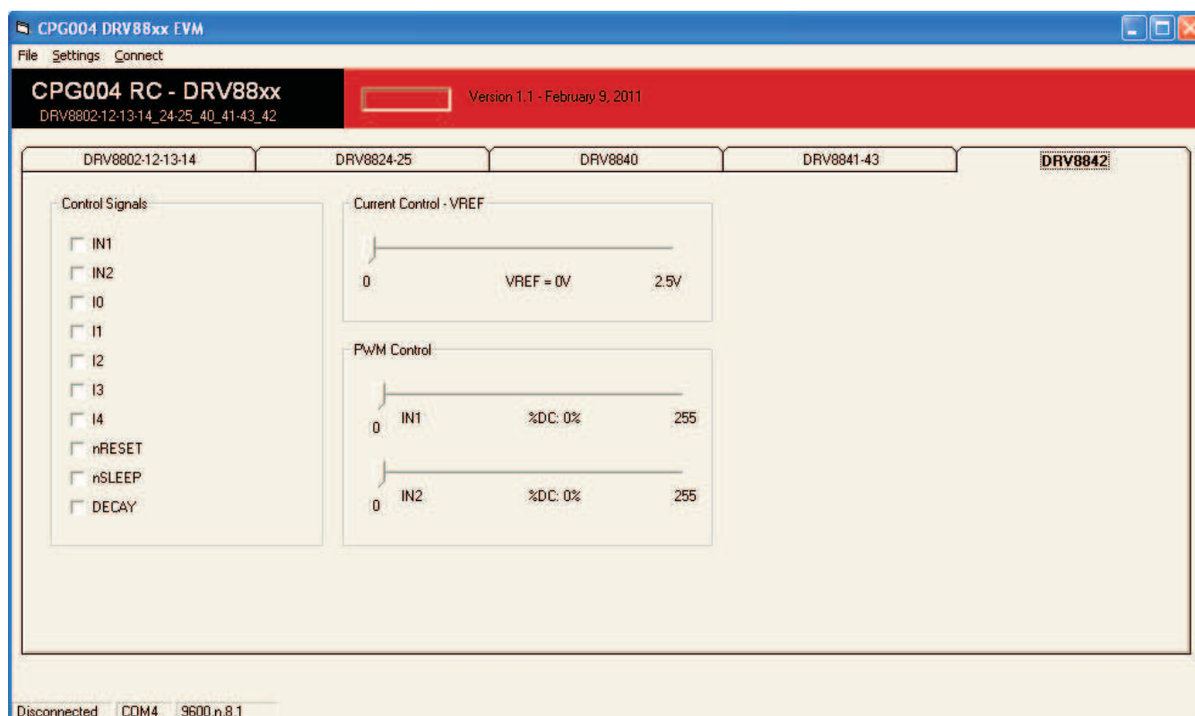
Figure 4. DRV8842 Tab
