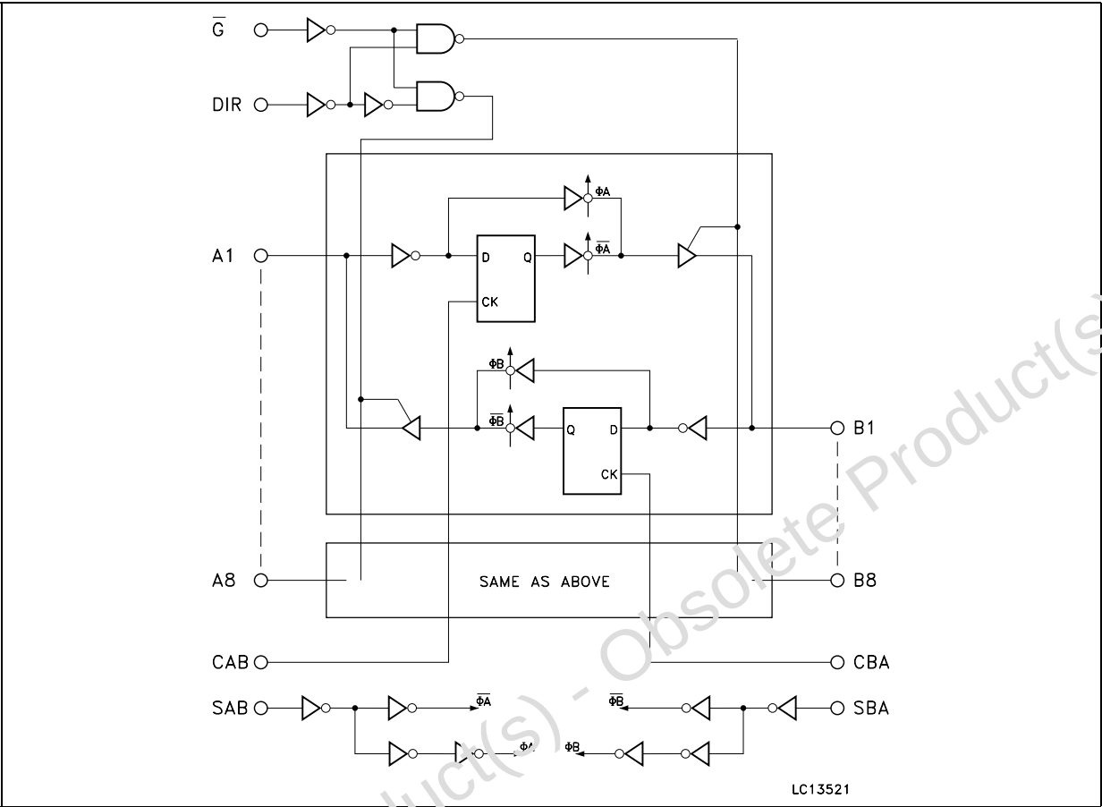
Figure 3: Logic Diagram
