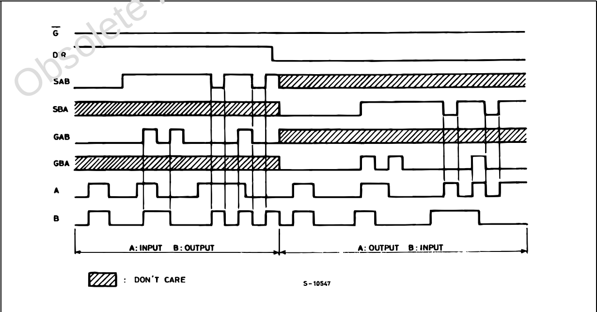
Figure 4: Timing Chart
