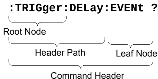
Figure 3-3: Command header
