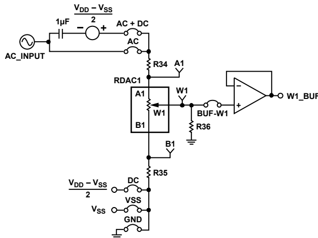
Figure 3. AC Signal Attenuator
