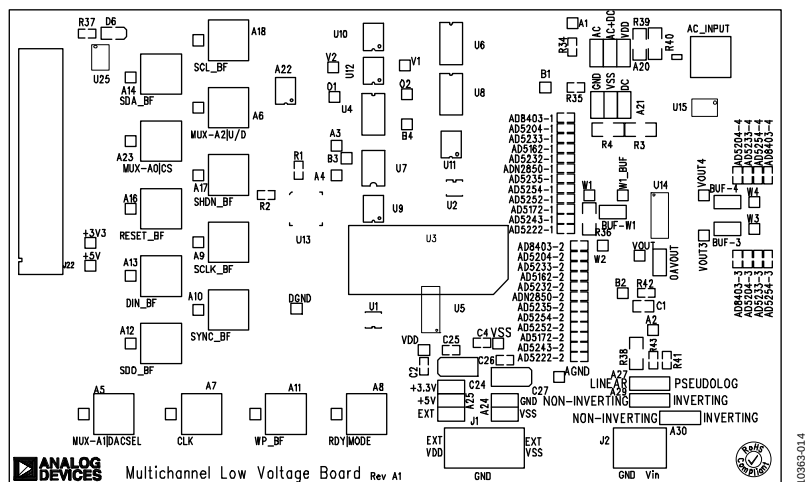
Figure 17. Component Side View
