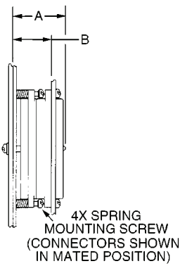
DLD Assembly Dimensions
