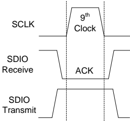
Figure 24: Valid Acknowledge
