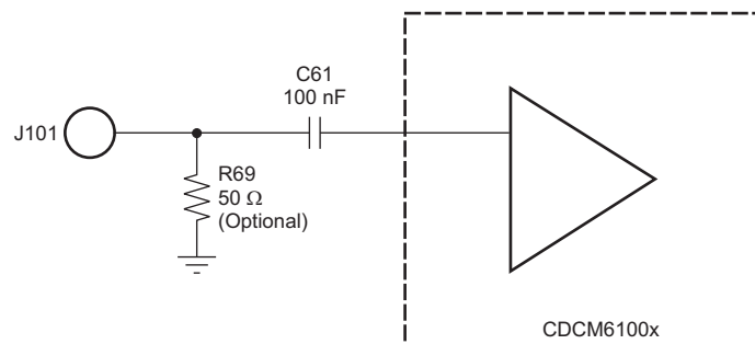
Figure 3. Single-Ended Connection Configuration
