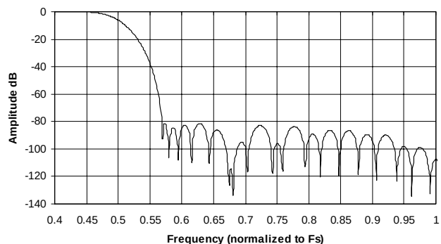
Figure 11. Double-speed Stopband
