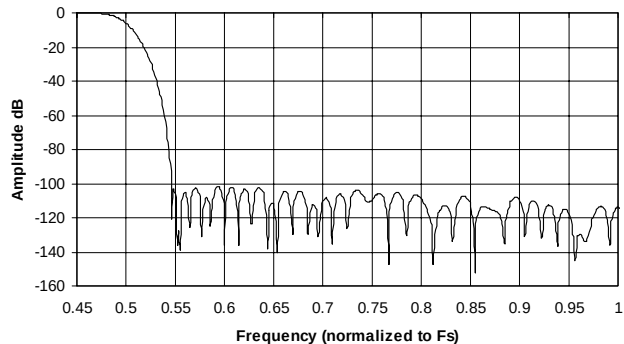
Figure 8. Single-speed Stopband Rejection
