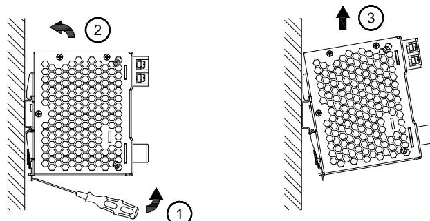
Fig. 2.2 Dismounting
