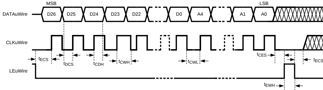
Figure 6. MICROWIRE Input Timing Diagram
