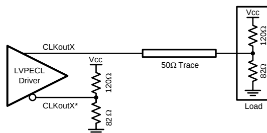
Figure 33. Single-Ended LVPECL Operation, DC Coupling, Thevenin Equivalent
