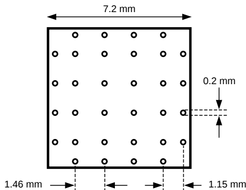
Figure 41. Recommended Land and Via Pattern
