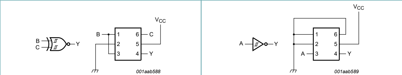
Fig. 10. 2-input XNOR gate
