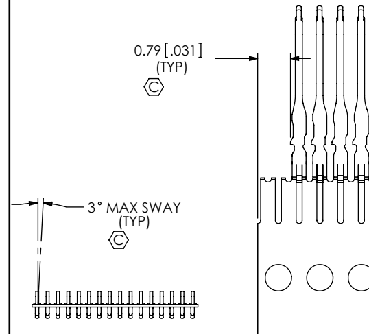
IN PROCESS 1 CUT C-247-XX.X-X CONTACT COMBS (ALL TAILS SAME DIRECTION)
