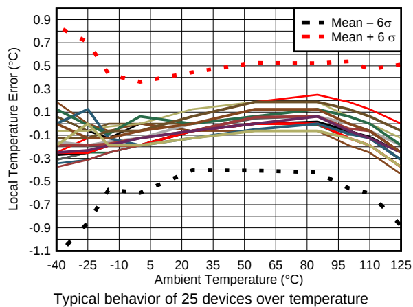
Figure 2. Local Temperature Error vs Ambient Temperature
