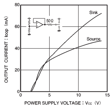
Fig.10 Power supply voltage vs. op-amp output drive voltage
