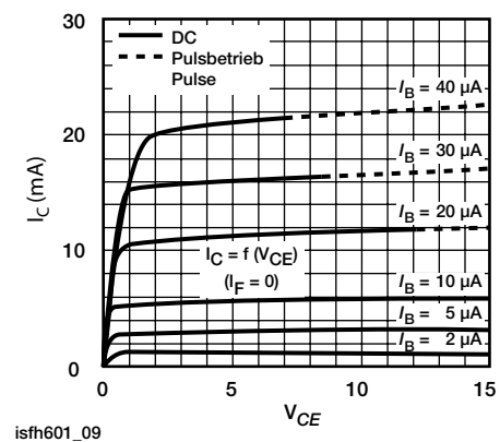
Fig. 9 - Transistor Characteristics
