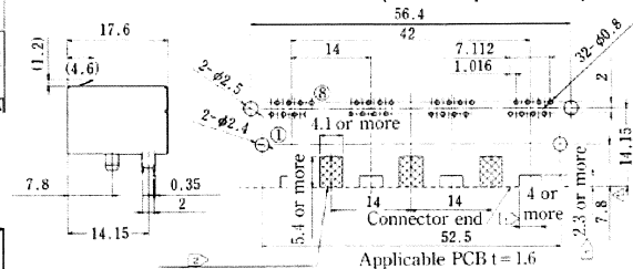
Reference mounting dimensions (PCB component side)
