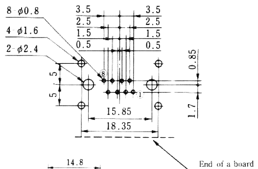
Board mounting dimensional drawing (connector side)
