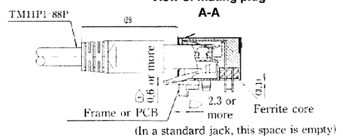
Reference mounting dimensions (PCB component side)
