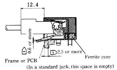
Reference mounting dimensions (PCB component side)
