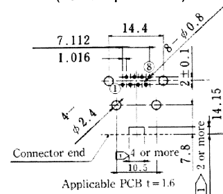
Reference mounting dimensions (PCB component side)
