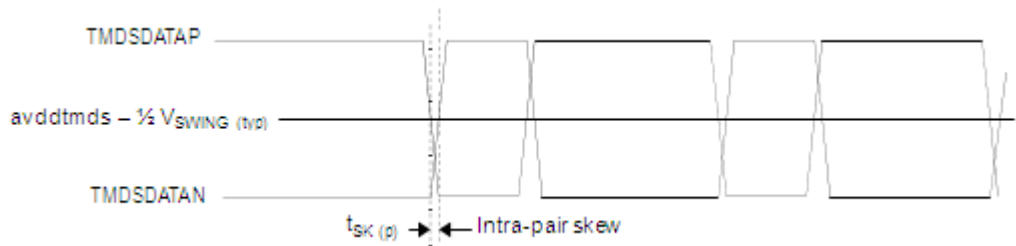
Figure 59. Intra-Pair Skew Definition
