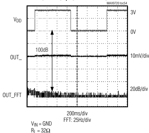
POWER-UP/DOWN WAVEFORM
