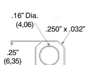
S 3 Solder Eye, extra large & quick connect
