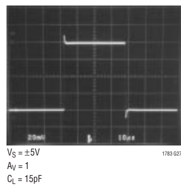
Small-Signal Response
