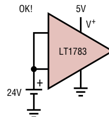
INPUT OVERVOLTAGE
