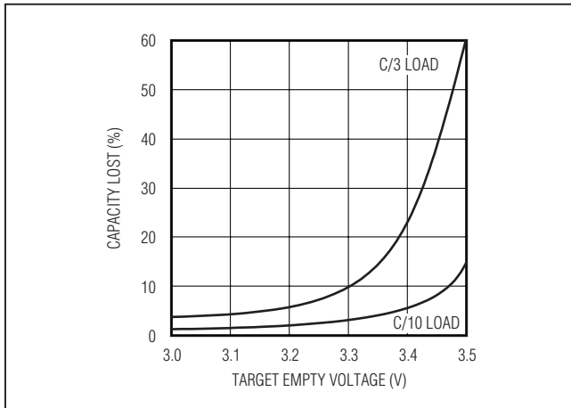
Figure 4. Increasing Empty Voltage Reduces Battery Capacity
