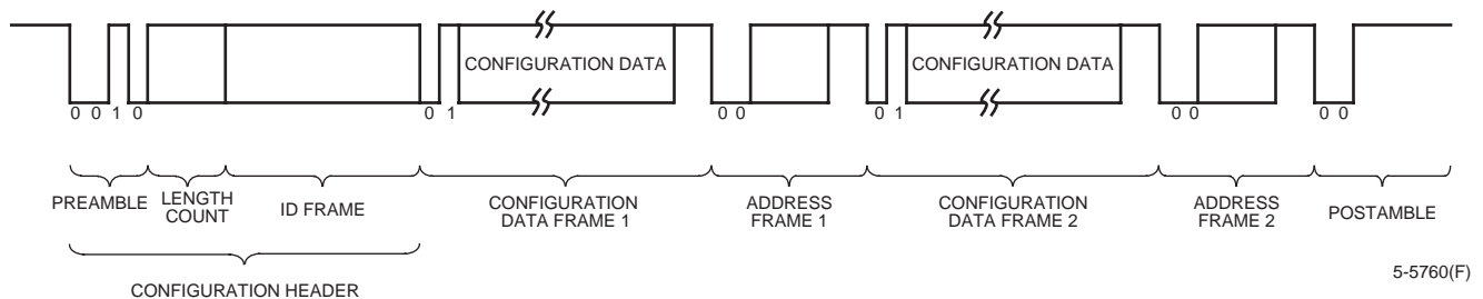
Figure 12. Serial Configuration Data Format—Explicit Mode
