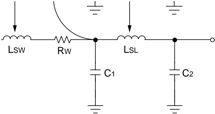
Figure 34. Package Parasitics
