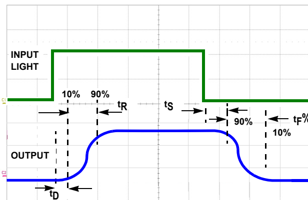
FIGURE 3. TIMING DIAGRAM
