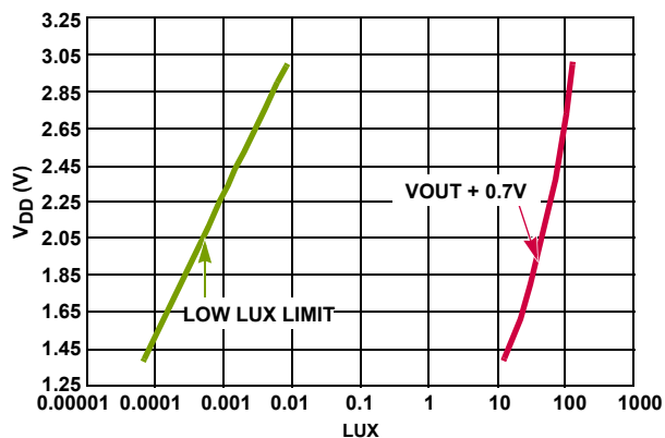
FIGURE 7. V_{DD} OPERATING RANGE (WHITE LED)
