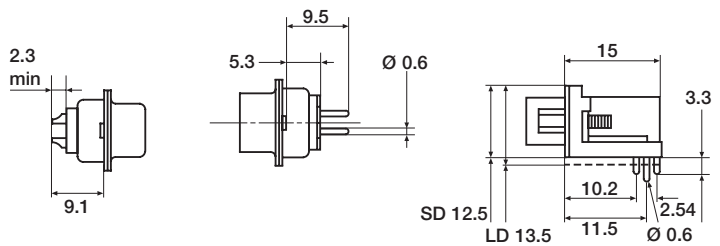
Solder Bucket
