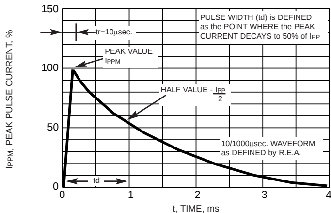
FIG. 3 - PULSE WAVEFORM
