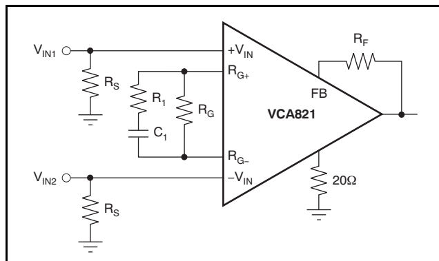
Figure 77. Differential Equalizer
