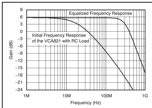
Figure 78. Differential Equalization of an RC Load
