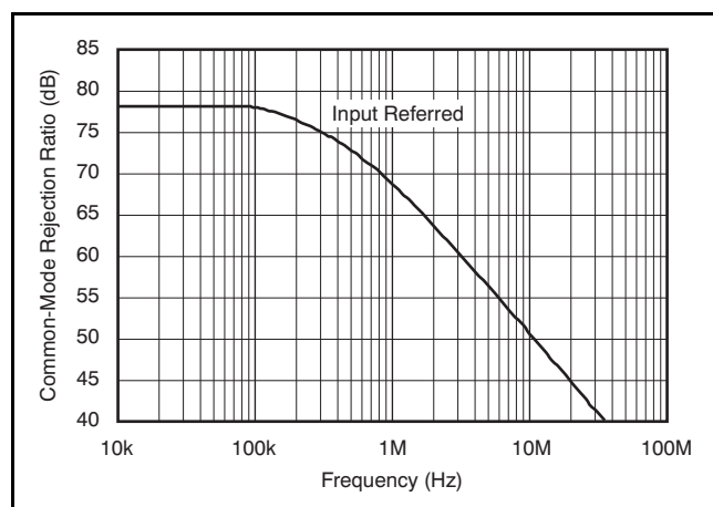
Figure 76. Common-Mode Rejection Ratio
